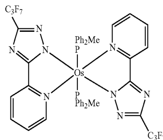
Os(hptz) 2 (PPh 2 Me) 2
